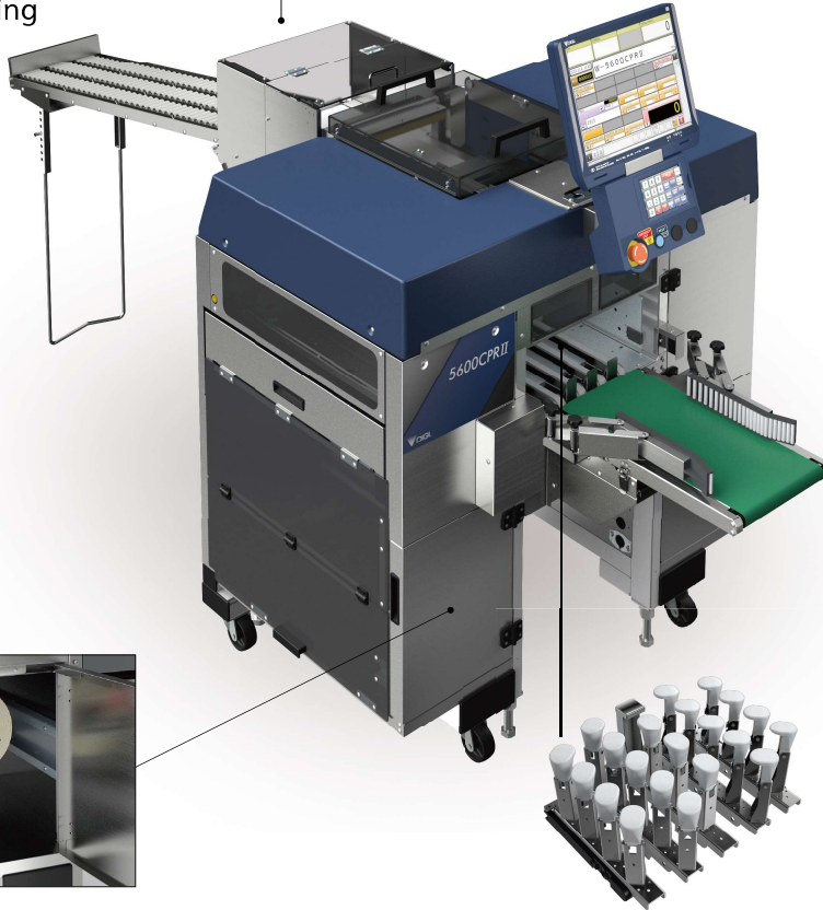
Quick, simple film loading using the new mechanism
